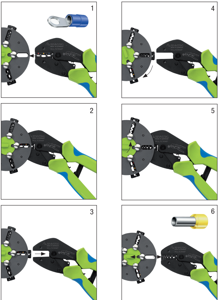
1-6: Fast, tool-free die change - one click and you're done
