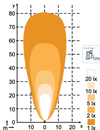
N73012 600 lm Flood TD US - T987-101B
