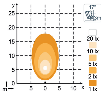
Flood - T980-102B 1000 Lumens
