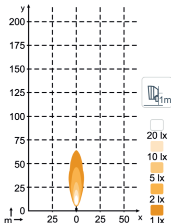
High Beam - T980-103B 1000 Lumens
