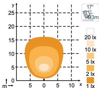
Wide Flood - T980-101B 1000 Lumens
