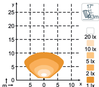
Super Wide - T980-104B 1000 Lumens
